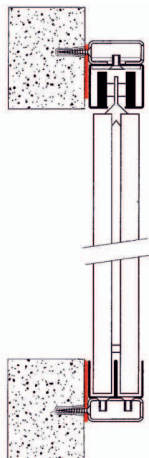
Face Fixed Side Elevation with Packer
