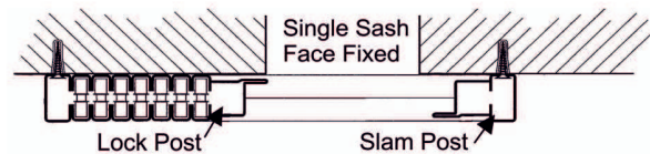
Face Fix Plan Views & Fixing Details
