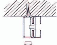
Face Fixed Side Frame Detail
