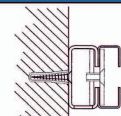
Fixing detail
