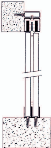
Face Fixed Side Elevation
