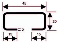
Fixing frame
