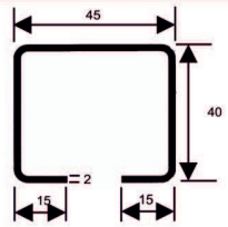
Top Track
