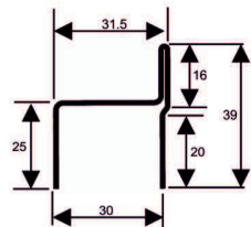
Lock Post
